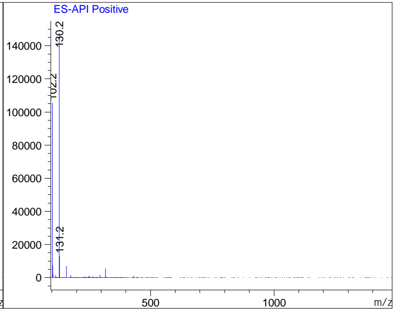
Ret. Time: 3.85
