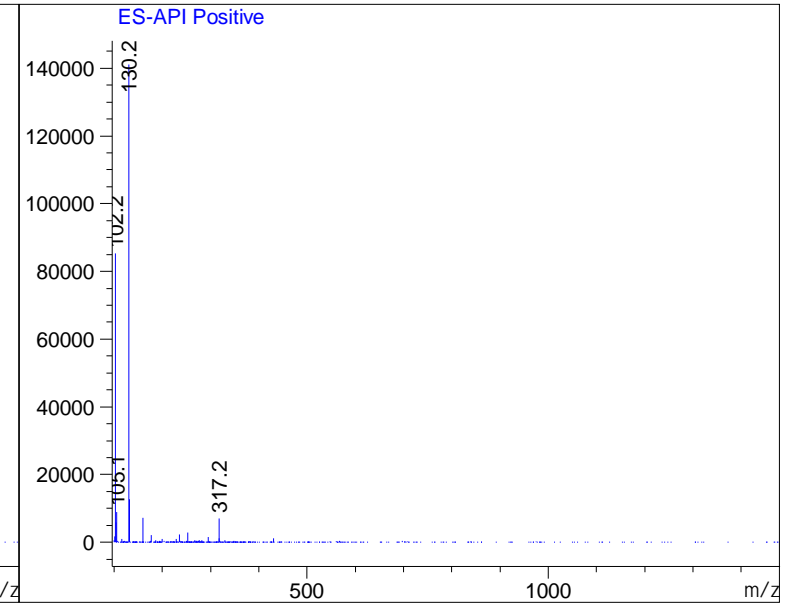
Ret. Time: 5.55
