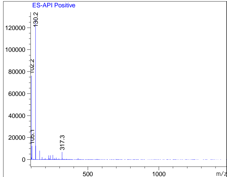
Ret. Time: 5.71
