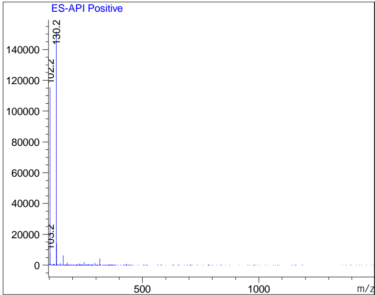
Ret. Time: 1.26
