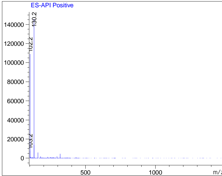
Ret. Time: 3.50
