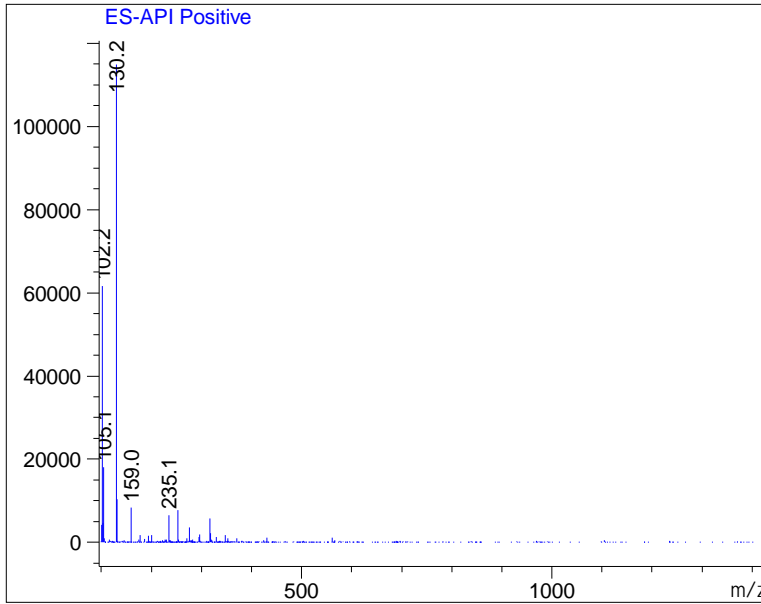
Ret. Time: 6.62
