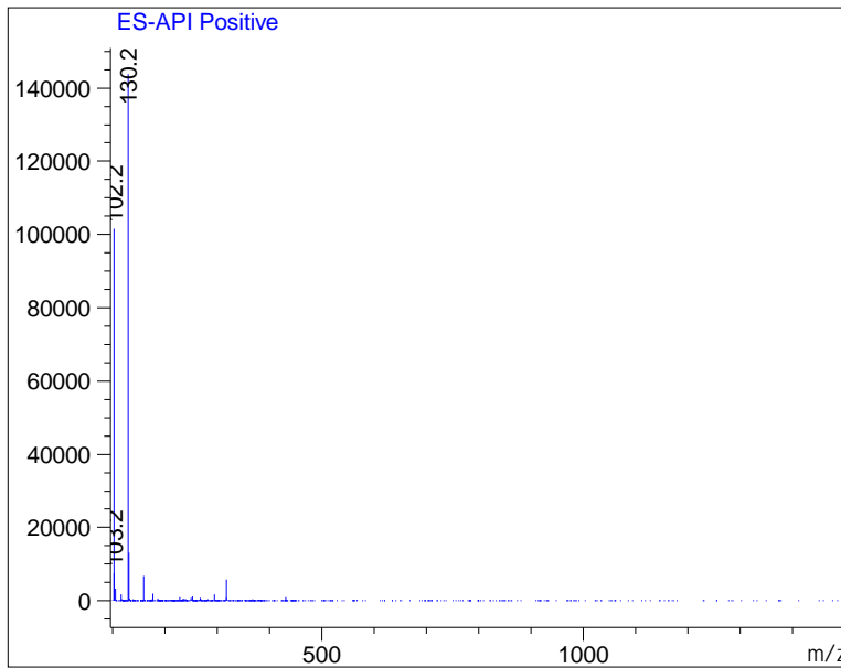
Ret. Time: 3.50
