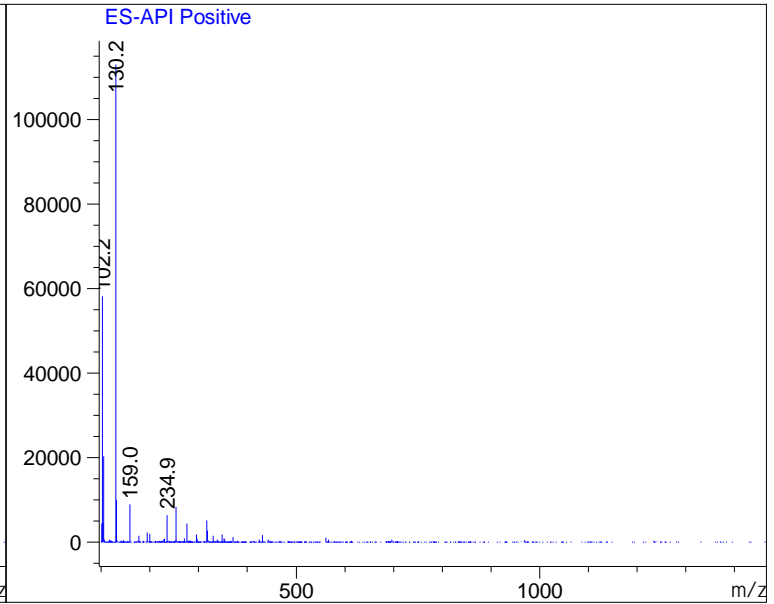
Ret. Time: 6.76
