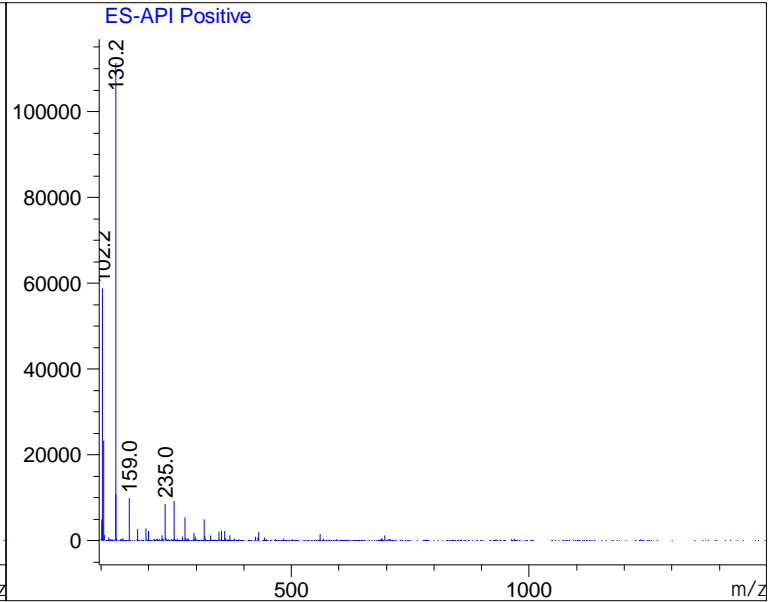
Ret. Time: 7.56
