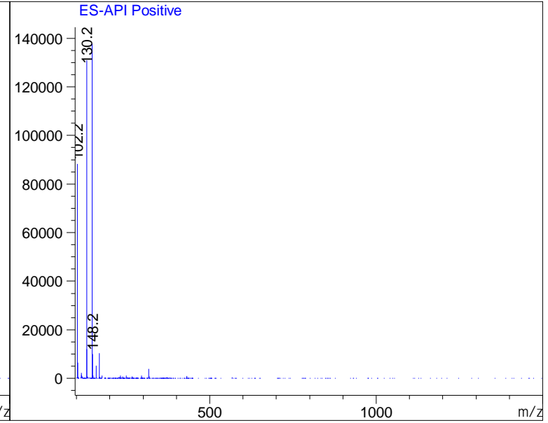
Ret. Time: 1.04
