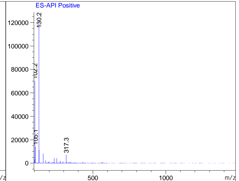
Ret. Time: 5.99
