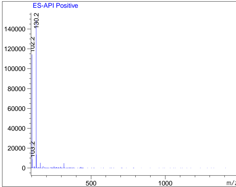
Ret. Time: 2.17
