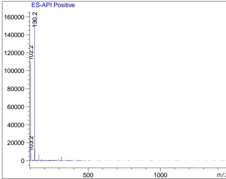
Ret. Time: 1.83
