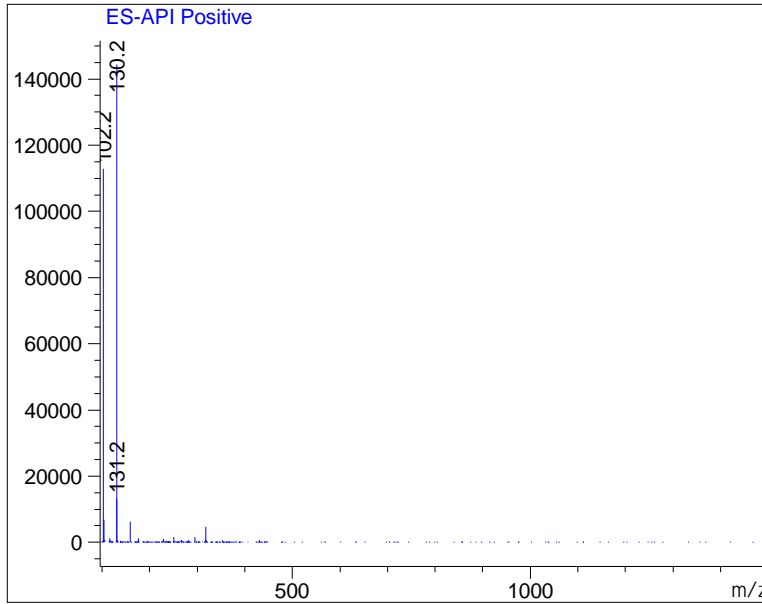
Ret. Time: 2.82
