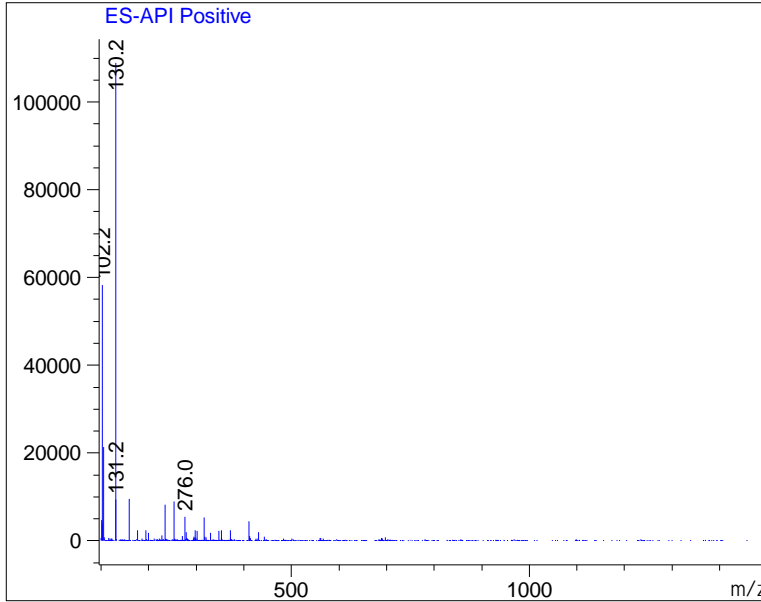
Ret. Time: 7.40
