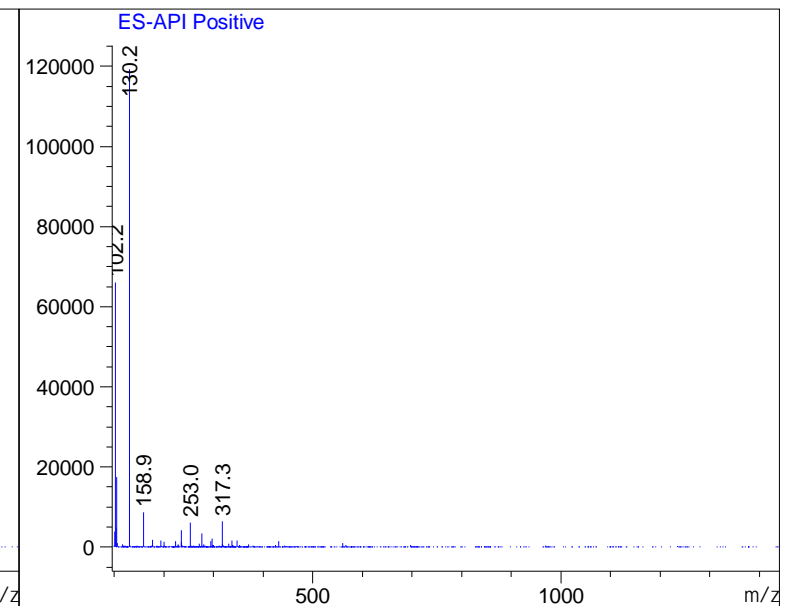
Ret. Time: 5.99
