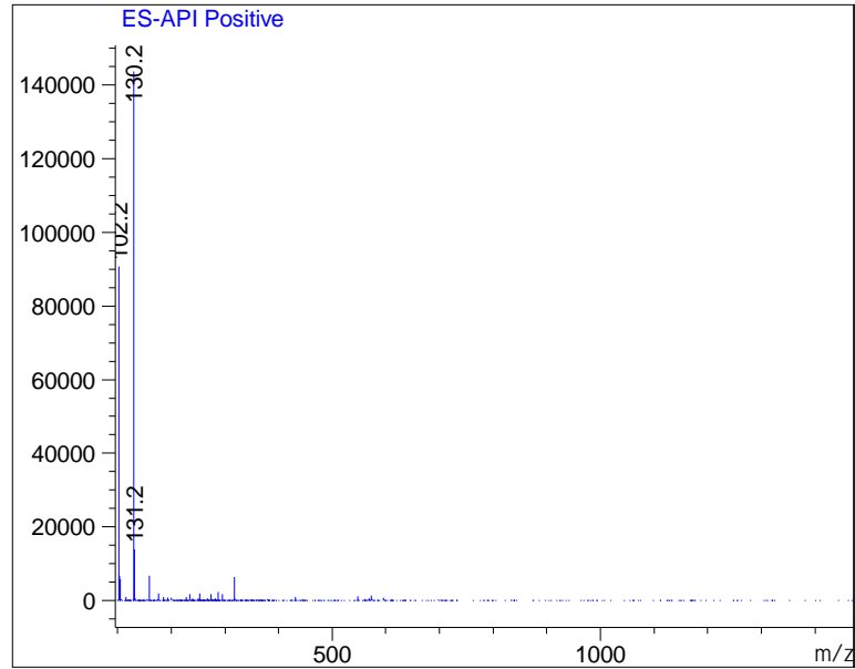
Ret. Time: 5.15
