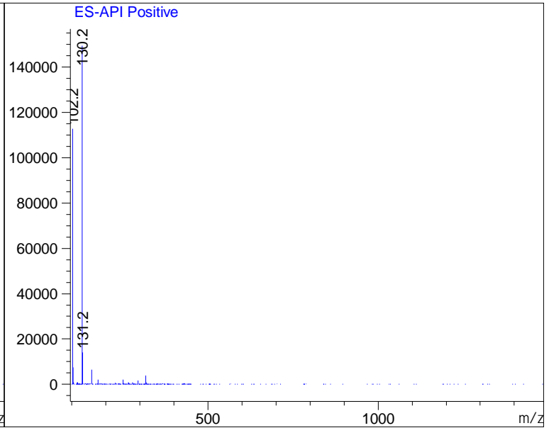
Ret. Time: 3.24
