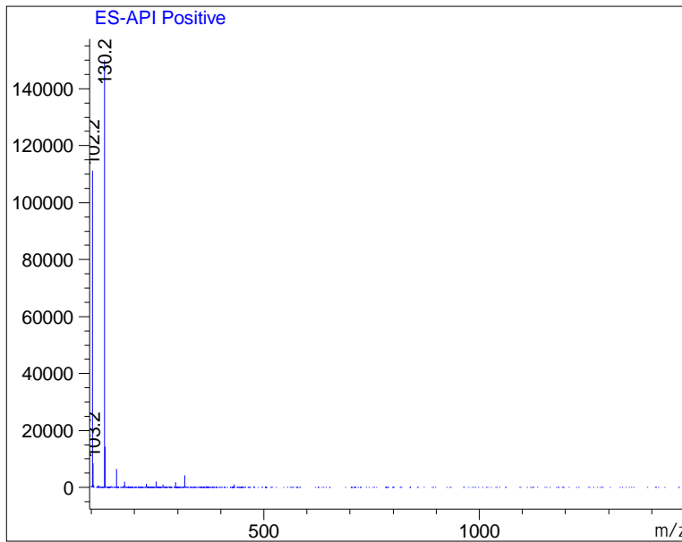
Ret. Time: 2.17
