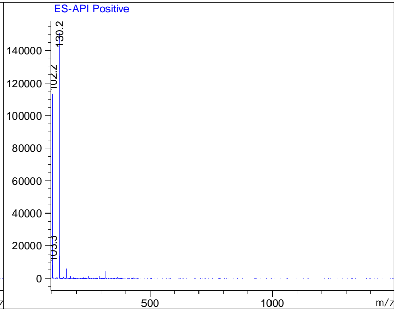
Ret. Time: 1.91
