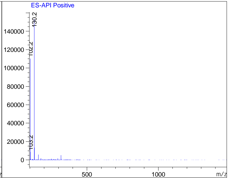
Ret. Time: 2.42
