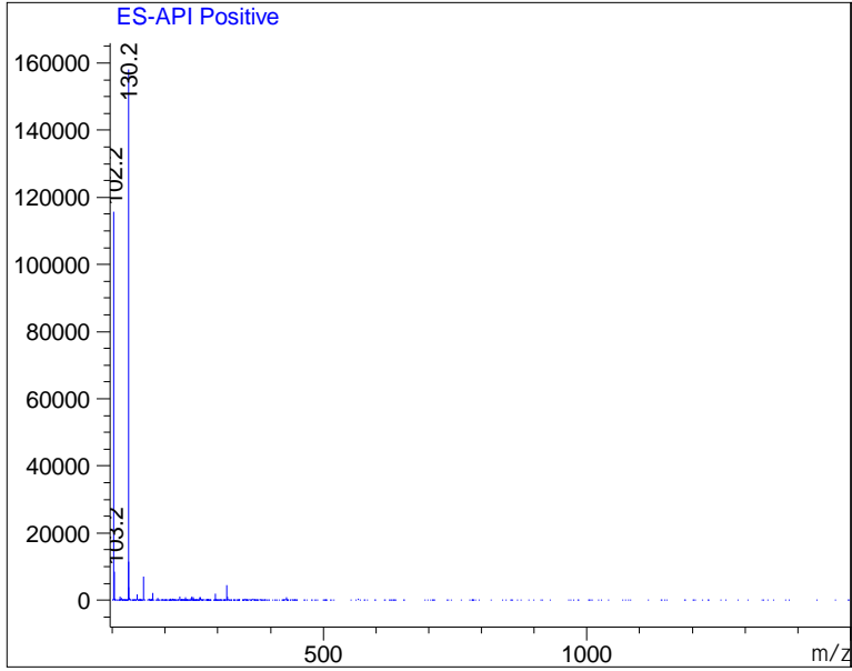
Ret. Time: 0.74
