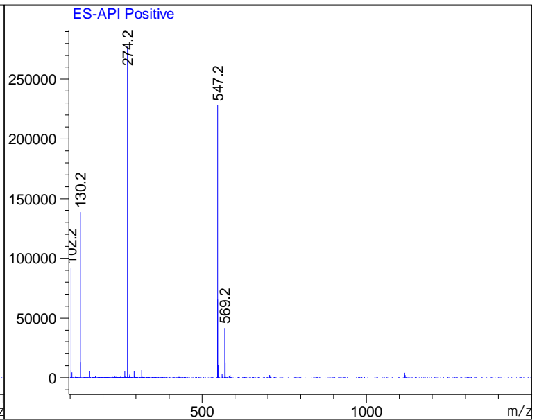
Ret. Time: 3.85
