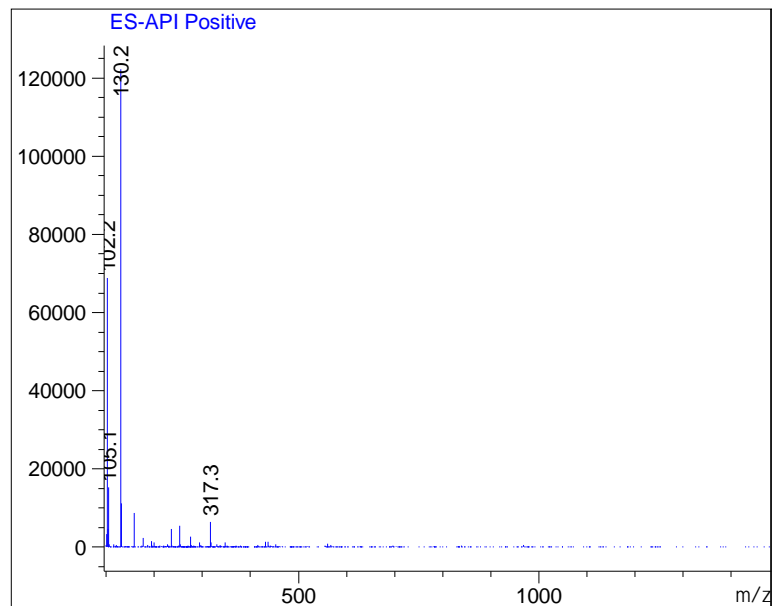
Ret. Time: 5.71
