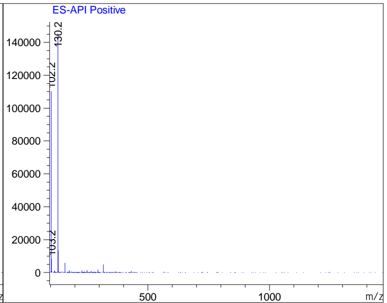
Ret. Time: 2.42
