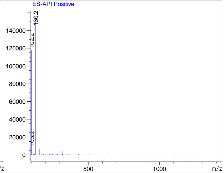
Ret. Time: 1.39
